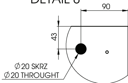
DETAIL 8
