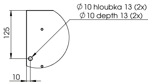
DETAIL 15
