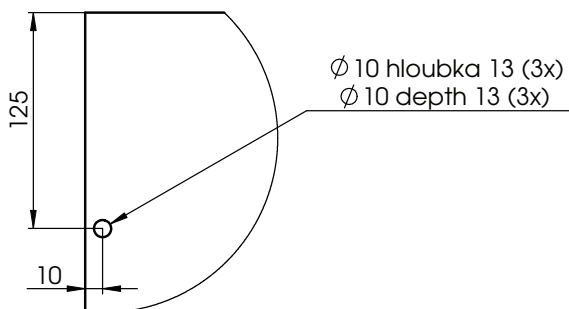
DETAIL 18
