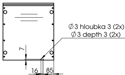
DETAIL 6
