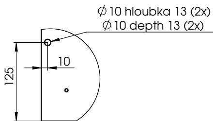
DETAIL 14
