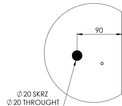
DETAIL 17
