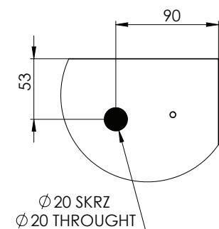
DETAIL 4
