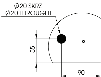
DETAIL 13
