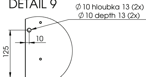
DETAIL 9
