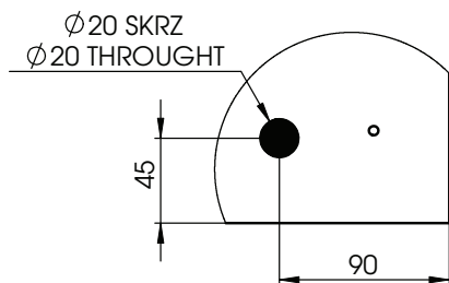
DETAIL 8
