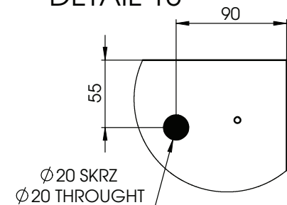
DETAIL 13
