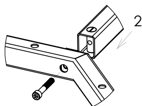
DETAIL 1.2
