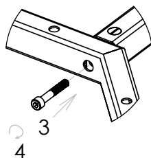
DETAIL 1.3
